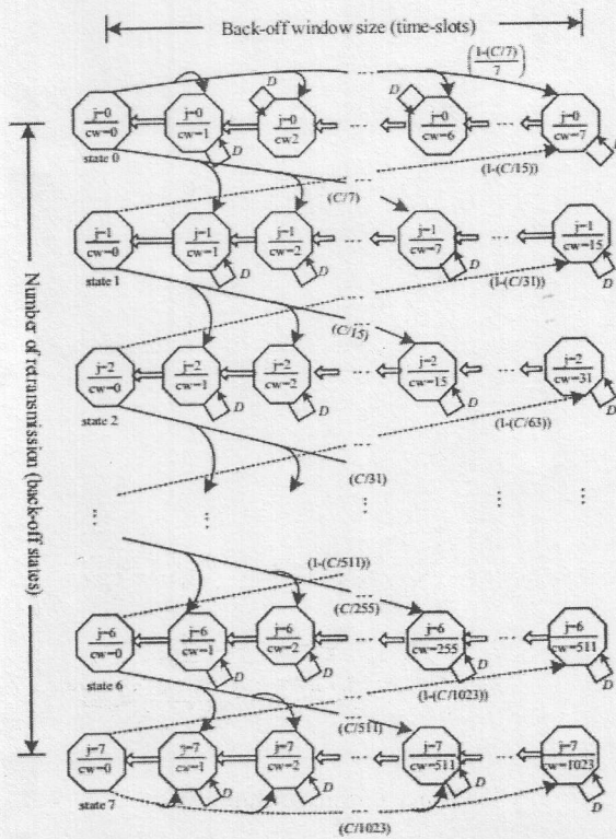
Figure 5 HBEIDD back-off algorithm
