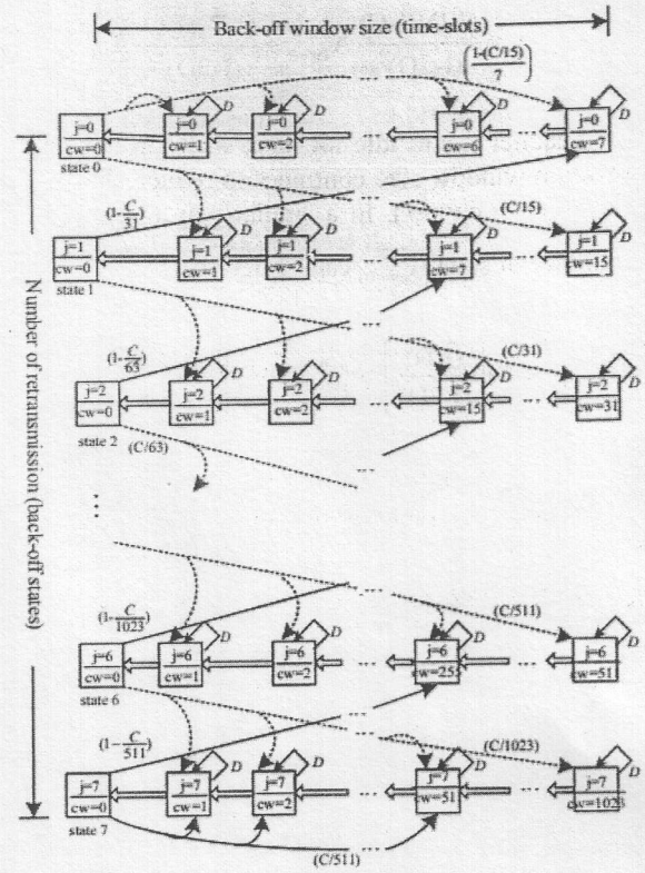
Figure 3 BEIHD back-off algorithm
