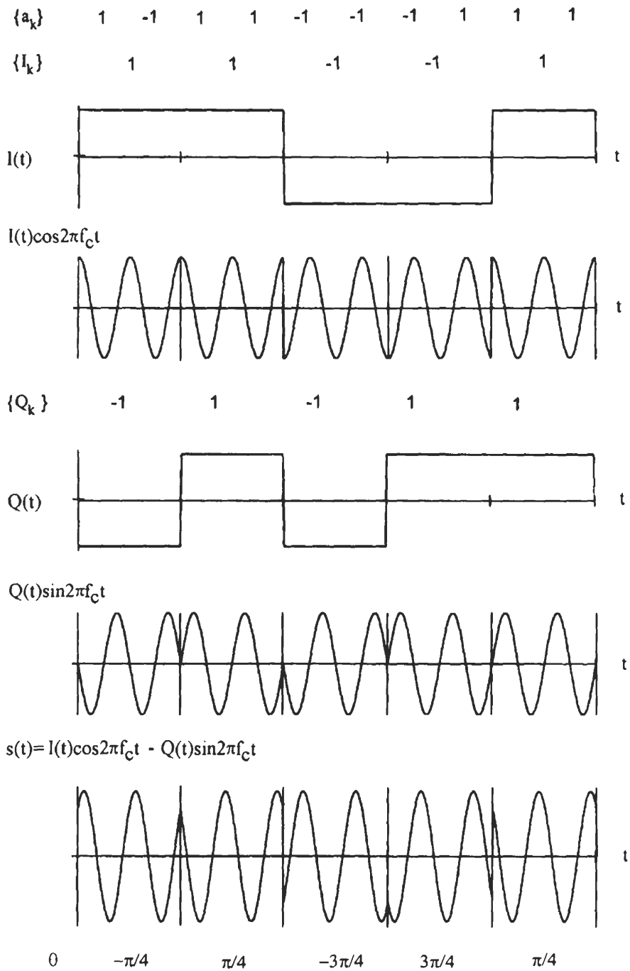
Figure 4.19 QPSK waveforms.
