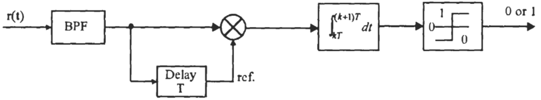
(b) DBPSK demodulator
