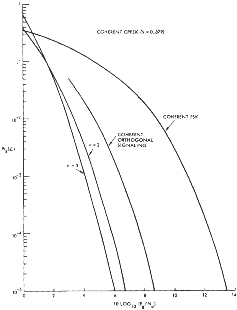
Figure 6.21 P_e for octal coherent CPFSK in comparison with coherent 8PSK and orthogonal signaling. From [22]. Copyright © 1976 IEEE.
