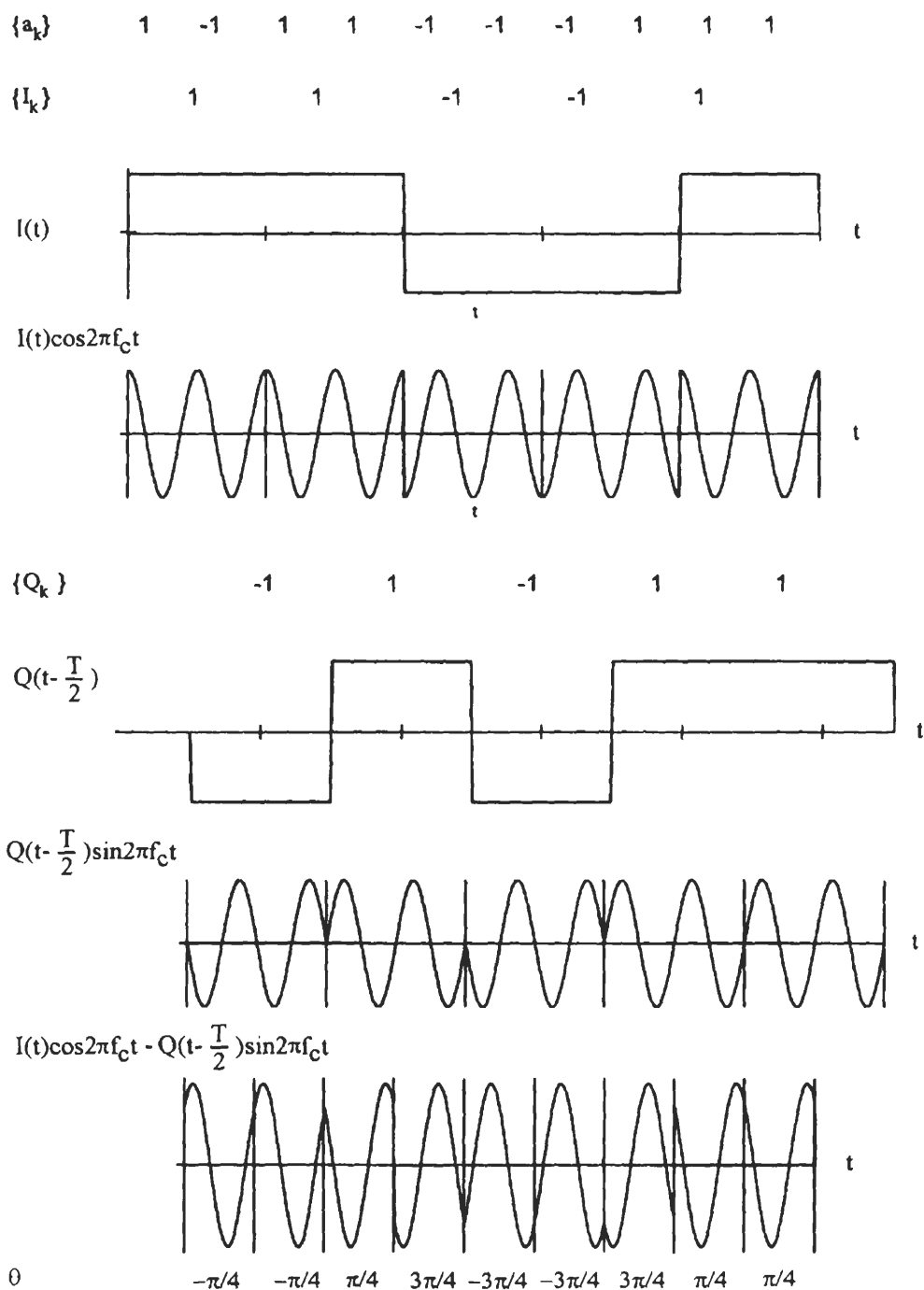
Figure 4.27 OQPSK waveforms.
