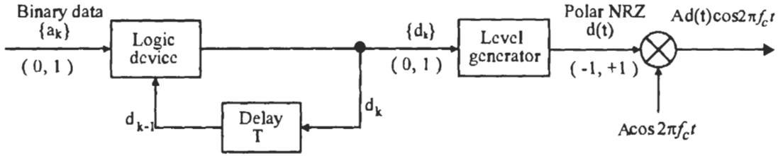
(a) DEBPSK modulator
