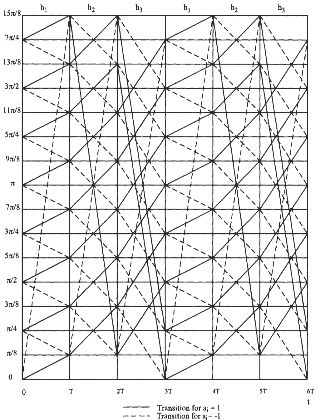
Figure 7.4 Phase trellis for H_3 = (1/8, 2/8, 3/8) binary CPFSK.
