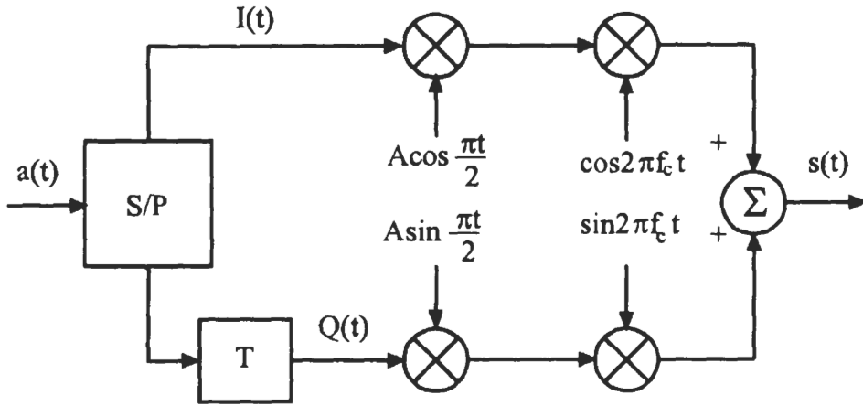
Figure 5.6 MSK modulator (l).
