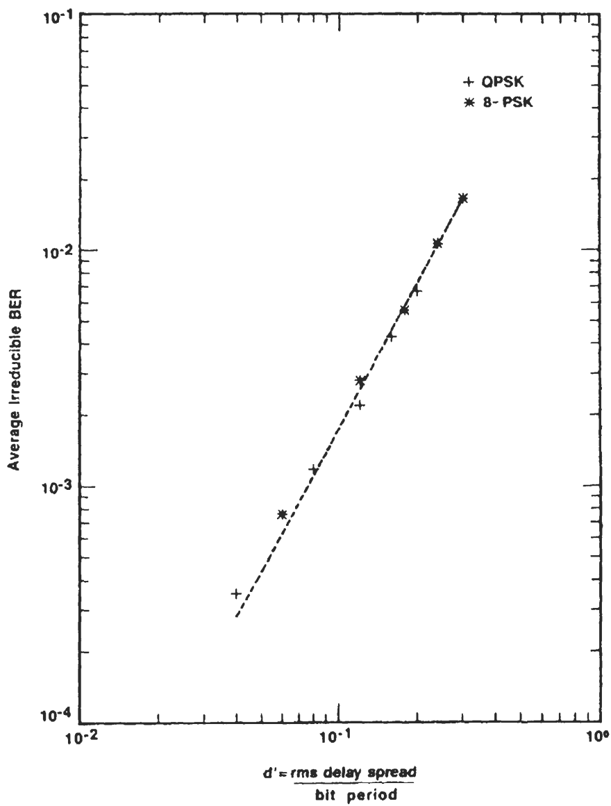
Figure 10.15 The irreducible BER performance for QPSK and 8-PSK. The parameter d' is the rms delay spread normalized by the bit period. From [9]. Copyright © 1987 IEEE.
