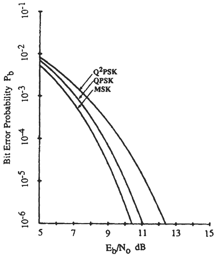
Figure 9.32 Bit error probability of Q 2 PSK, QPSK and MSK in a bandlimited channel. Bandlimiting filter is six-order Butterworth with 3 dB bandwidth equal to 1.2/T . From [12]. Copyright © 1989 IEEE.
