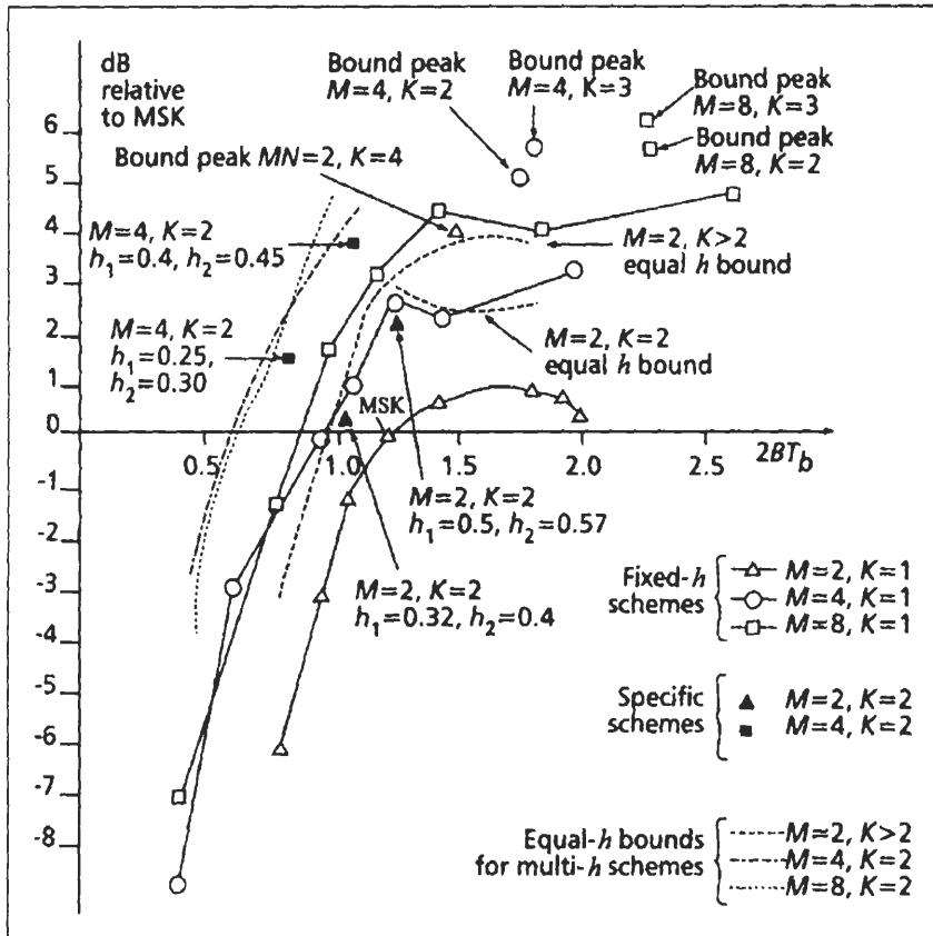
Figure 7.12 Power bandwidth trade-off for M-ary 1REC MHPM schemes. The bandwidth is the -20 dB (99%) out-of-band power bandwidth. All schemes are compared at equal bit rate. From [9]. Copyright © 1982 IEEE.
