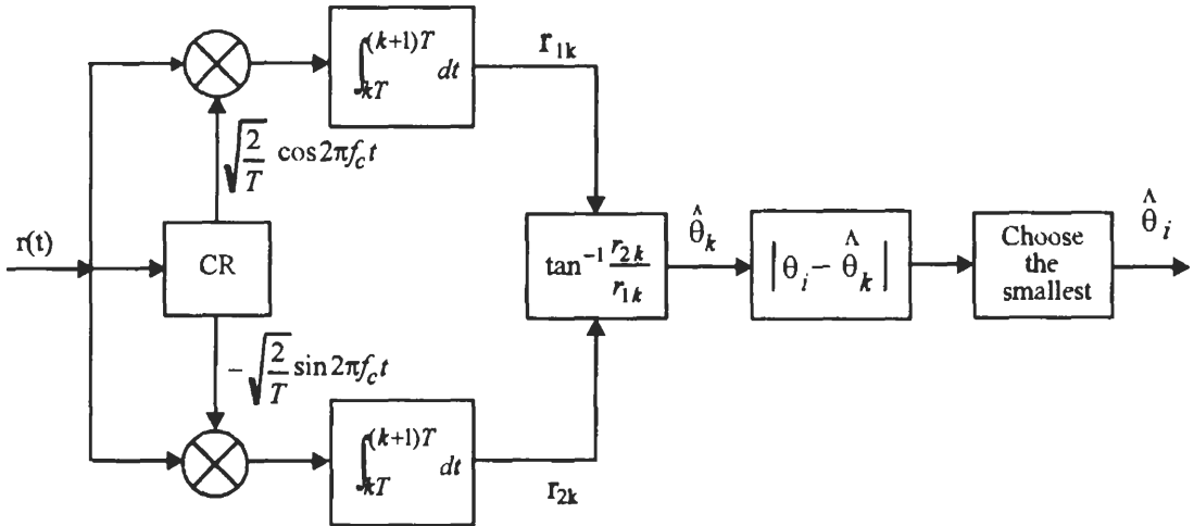
Figure 4.11 Coherent MPSK demodulator using two correlators.
