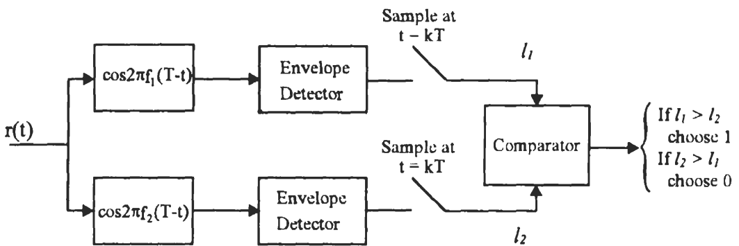
Figure 3.10 FSK noncoherent demodulator: matched filter implementation.
