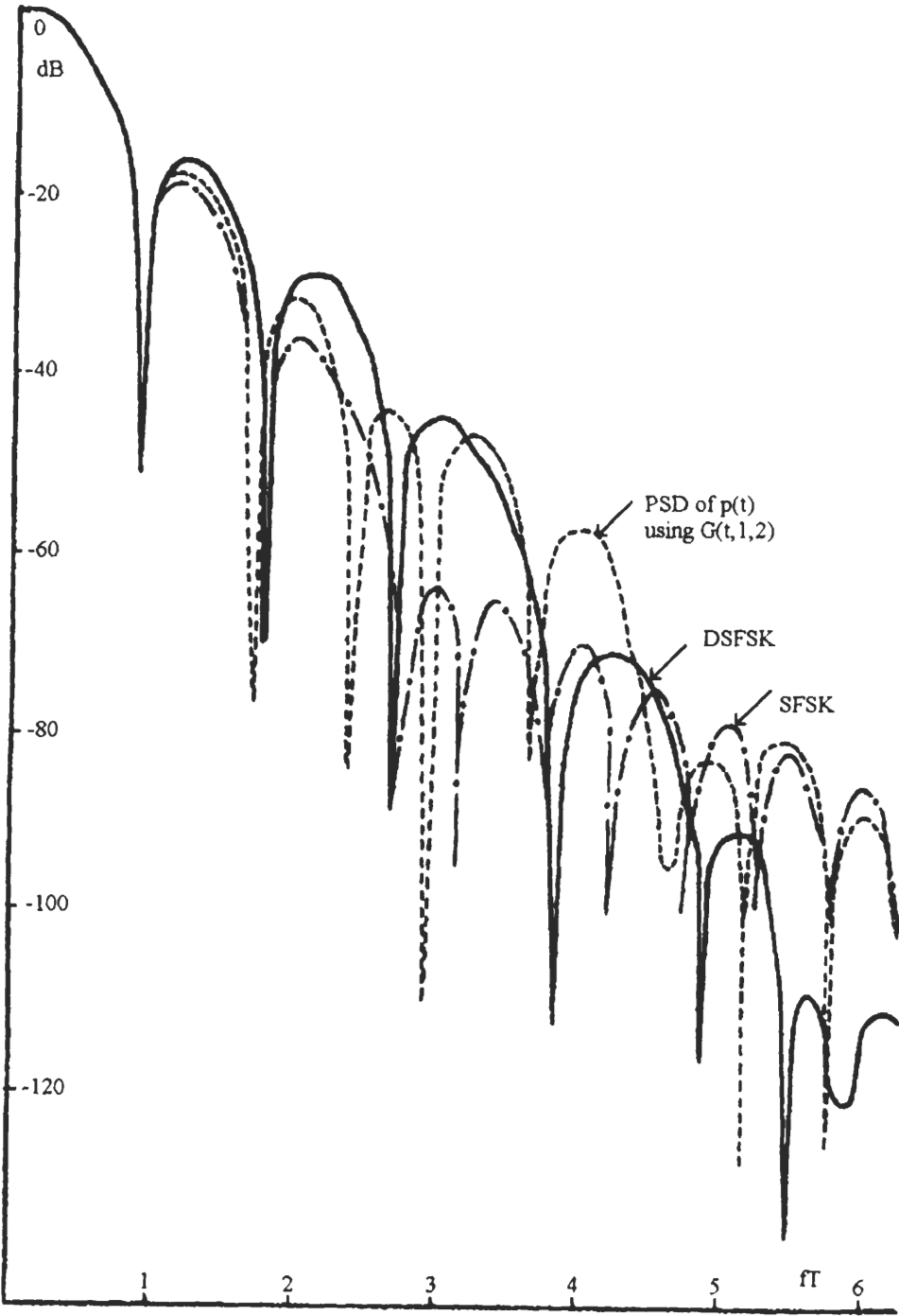
Figure 5.31 Power spectra. From [15]. Copyright © 1979 IEEE.
