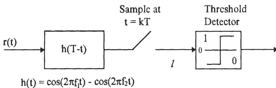
Figure 3.7 Coherent FSK demodulator: matched filter implementation.
