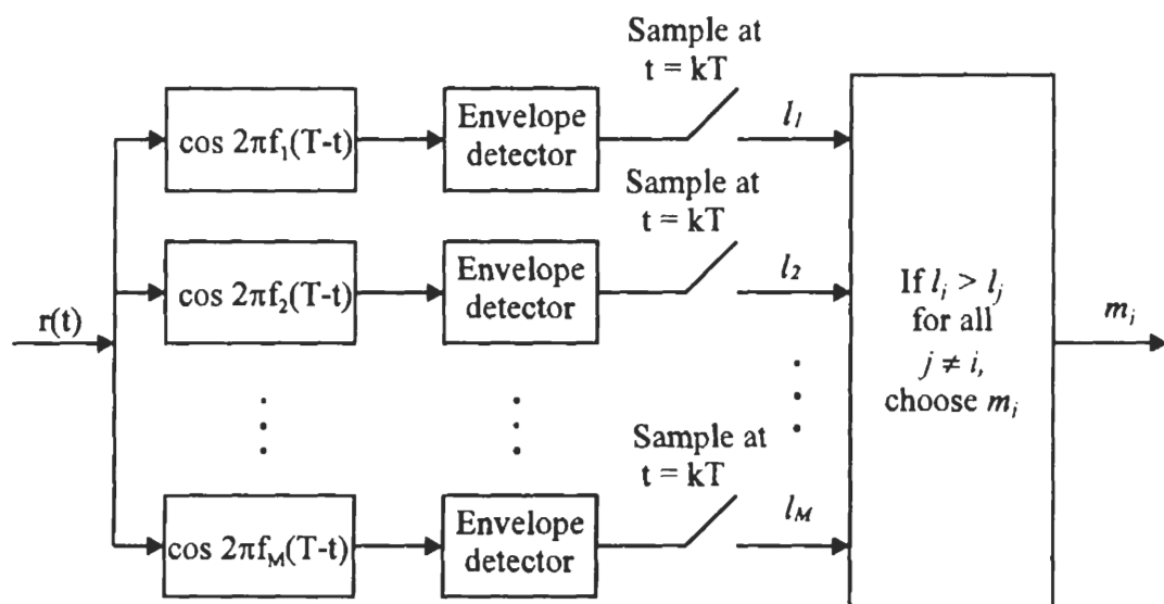
Figure 3.23 Noncoherent MFSK demodulator: matched filter-envelope detector implementation.
