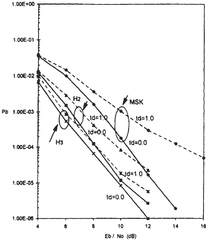
Figure 10.26 Comparison of MSK, H_2 = (2/4, 3/4) , and H_3 = (4/8, 5/8, 6/8) in Rician channel ( K = 10\text{dB} , f_d = 0.2 ). From [14]. Copyright © 1997 IEEE.
