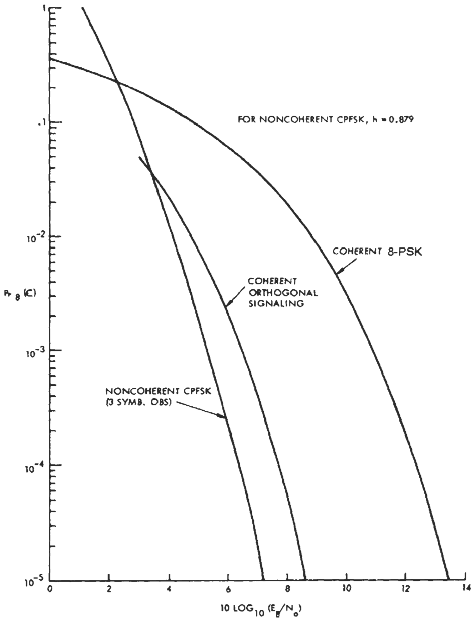
Figure 6.25 P_e of 8-ary noncoherent CPFSK in comparison with coherent 8PSK and coherent orthogonal signaling. From [22]. Copyright © 1976 IEEE.
