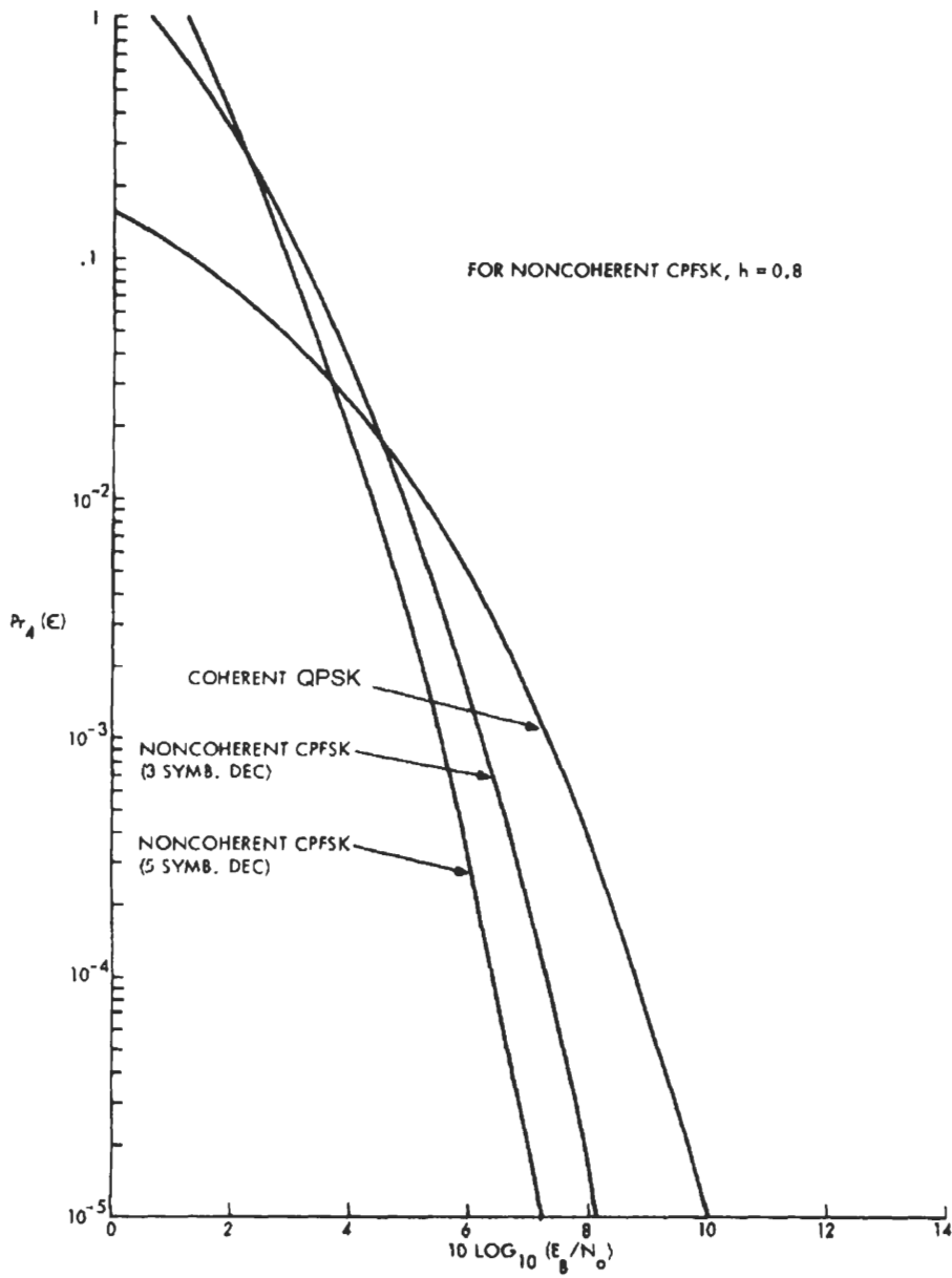
Figure 6.24 P_e of 4-ary noncoherent CPFSK in comparison with coherent QPSK. From [22]. Copyright © 1976 IEEE.
