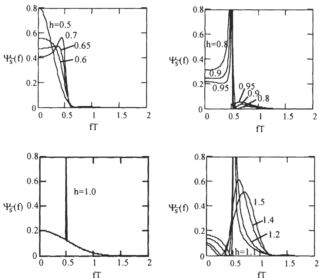
Figure 3.12 PSD of MFSK: M = 2 . After [1].
