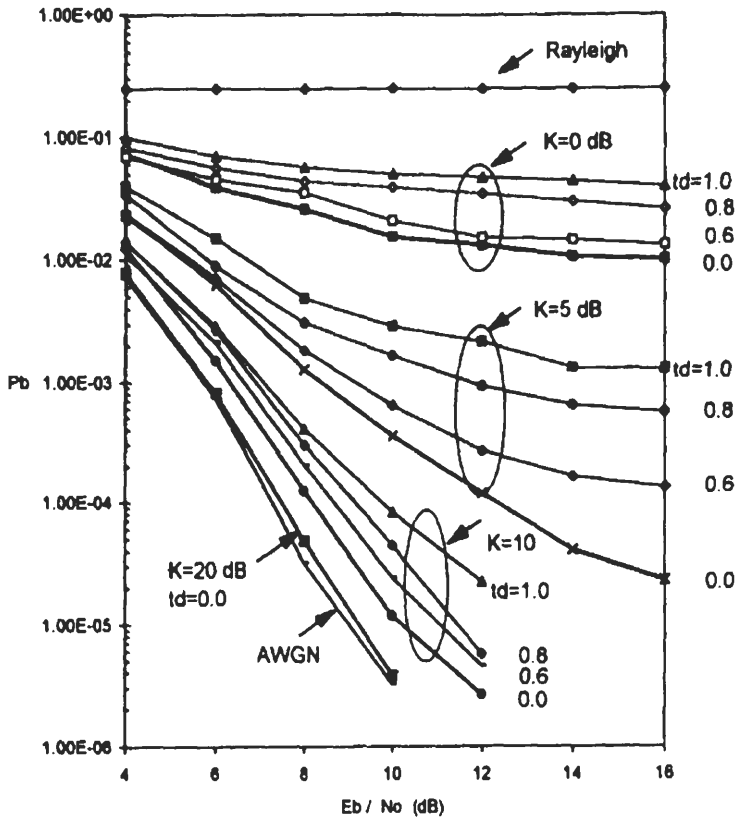
Figure 10.24 Performance of IREC-MHPM H_2 = (2/4, 3/4) in Rayleigh, Rician, and AWGN channels for various values of K and t_d ( f_d = 0.2 ). Rayleigh channel is approximated by K = -200 dB, and no synchronization is done for the Rayleigh fading signal. From [14]. Copyright © 1997 IEEE.
