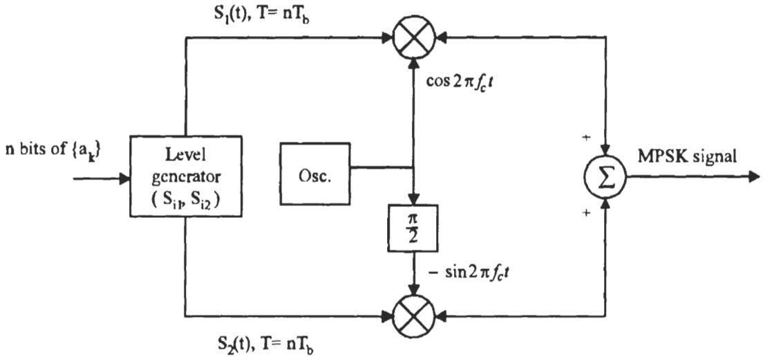
Figure 4.10 MPSK modulator.
