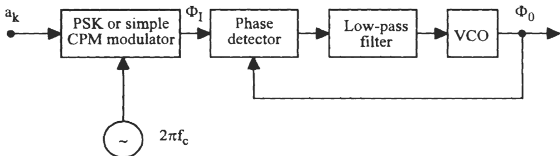
Figure 6.15 PLL implementation of CPM modulator. From [9] Copyright 1986 © Plenum.
