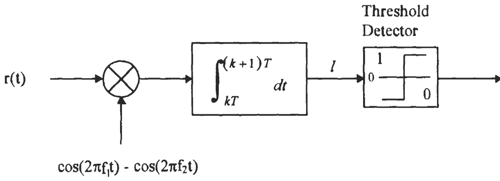
Figure 3.6 Coherent FSK demodulator: one correlator implementation.
