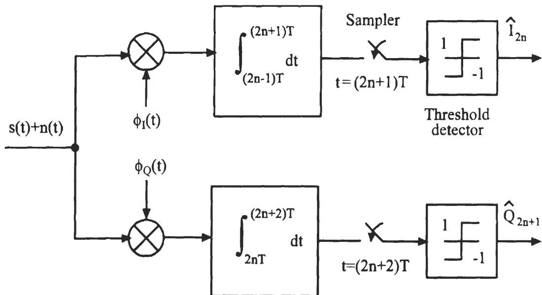
Figure 5.9 MSK demodulator (I).
