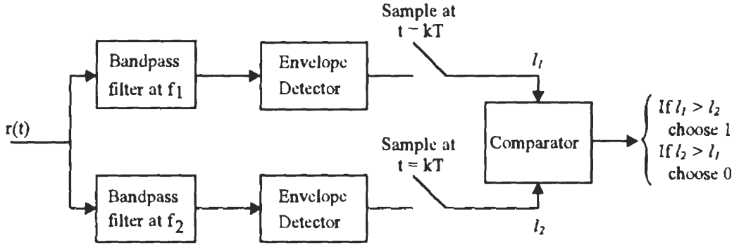
Figure 3.11 FSK noncoherent demodulator: bandpass filter implementation.
