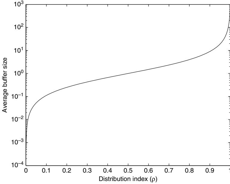
Fig. 7.2 Average queue size versus the distribution index \rho for the M/M/1 queue
