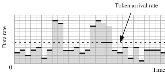
Fig. 8.6 Control of data rate by the token bucket algorithm. Data rate at the input is indicated by the grey areas, data rate at the output is indicated by the black lines and the dashed line is the token issue rate
