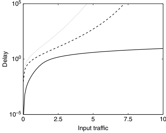
Fig. 10.35 Delay for the 1-persistent IEEE 802.11/PCF protocol versus the average input traffic when N = 10 . The solid line is the delay of 1-persistent IEEE 802.11/PCF, the dashed line represents the delay of slotted ALOHA, and the dotted line represents the delay of pure ALOHA
