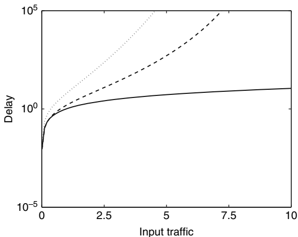
Fig. 10.14 Frame delay for the CSMA/CA protocol versus the average input traffic for the case n = 50 and N = 10 . The solid line is the delay of CSMA/CA, the dashed line represents the delay of slotted ALOHA, and the dotted line represents the delay of pure ALOHA
