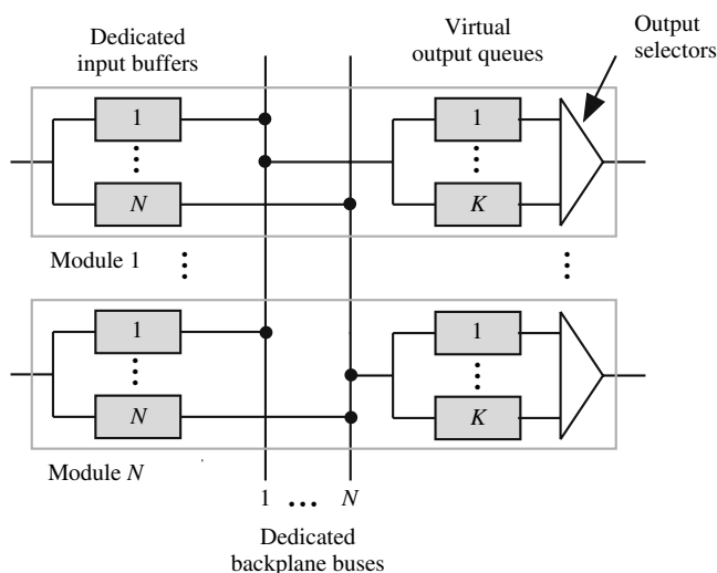
Fig. 16.2 The virtual routing, virtual queuing (VRQ) high-performance switch
