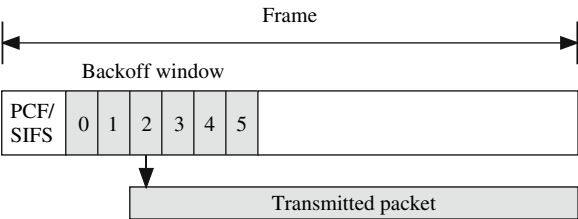
Fig. 10.16 DCF part of the IEEE 802.11 frame
