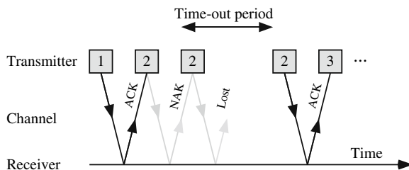
Fig. 9.1 Stop-and-wait ARQ protocol
