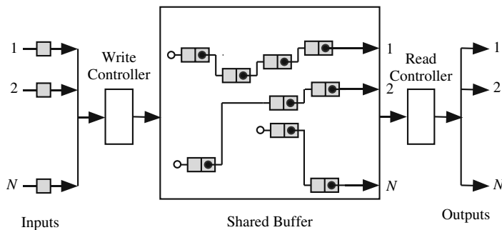
Fig. 15.7 The shared buffer switch
