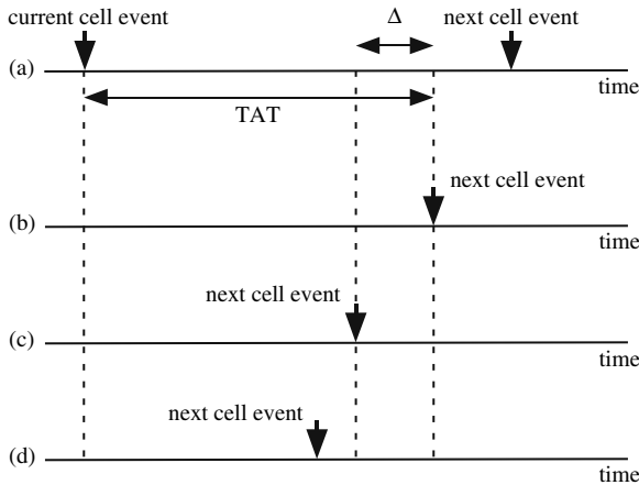
Fig. 8.12 Different cases for cell arrival in the VS algorithm. (a) t > \text{TAT} and cell is conforming. (b) t = \text{TAT} and cell is conforming. (c) t = \text{TAT} - \Delta and cell is conforming. (d) t < \text{TAT} - \Delta and cell is nonconforming
