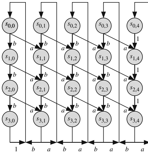
Fig. 7.9 State transition diagram for the discrete-time M/D/1/B queue
