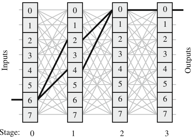
Fig. 14.23 Paths chosen in the ILN network to route a packet from input at row 6 to output at row 0
