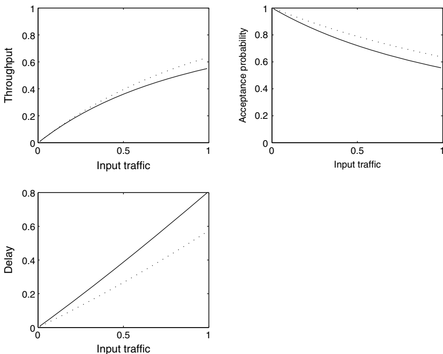
Fig. 14.25 Variation of the throughput, the packet acceptance probability, and the delay with the input traffic when N = 64 for the ILN network ( solid line ) and the similar-sized crossbar network ( dotted line )
