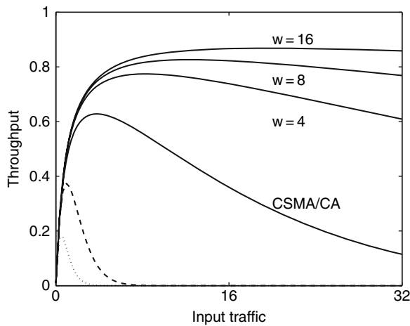
Fig. 10.21 Throughput for the IEEE 802.11/DCF protocol versus the average input traffic when n = 10 and N = 32 and w = 4, 8 , and 16. Dashed line represents the throughput of slotted ALOHA and the dotted line represents the throughput of pure ALOHA
