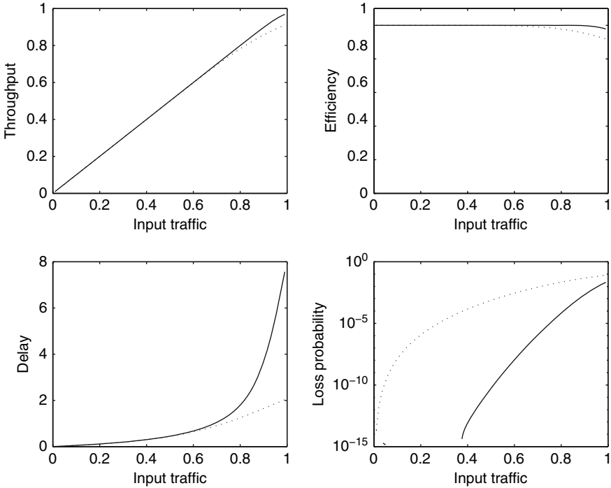
Fig. 15.9 Performance of a shared buffer switch versus the input traffic. Switch throughput, efficiency, delay, and loss probability are plotted against input traffic. The solid line is for a switch with B = 16 and the dotted line is for a switch with B = 4
