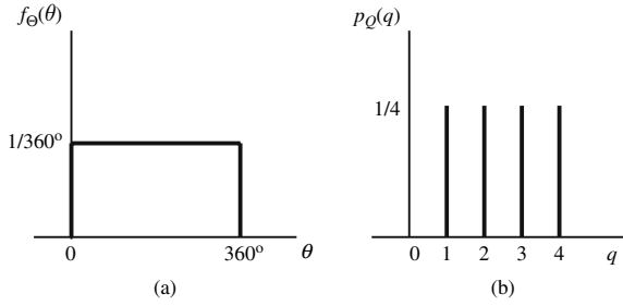
Fig. 1.6 Continuous and discrete random variables. (a) pdf for the continuous case. (b) pmf for the discrete case
