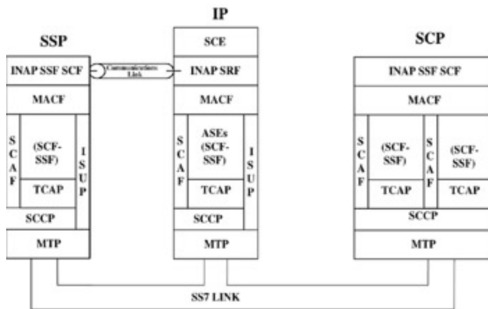
Figure 4.3: AIN protocol stack
