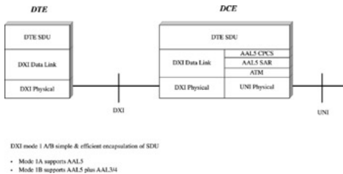
Figure 12-14: DXI modes 1A and 1B
