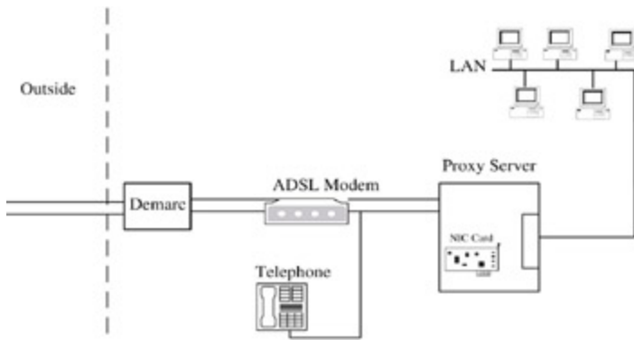
Figure 16-13: The proxy server in lieu of a single attached PC
