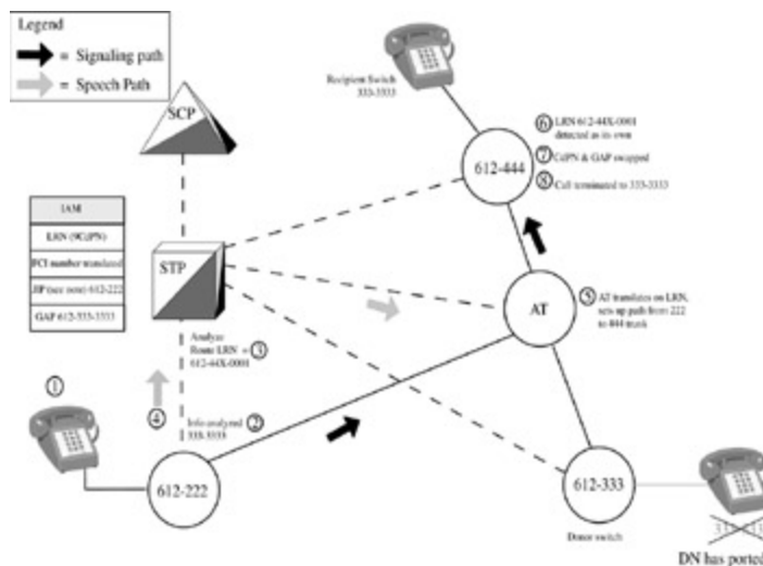
Figure 5-4: The LRN in use
