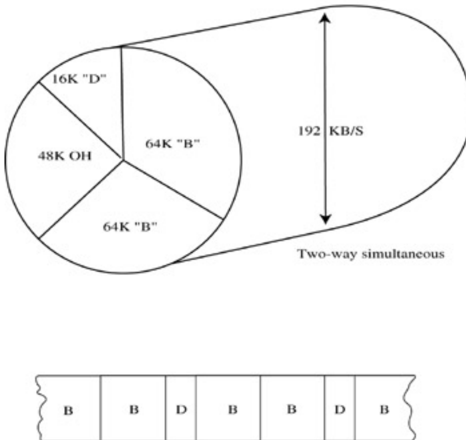
Figure 9-1: BRI bandwidth allocation
