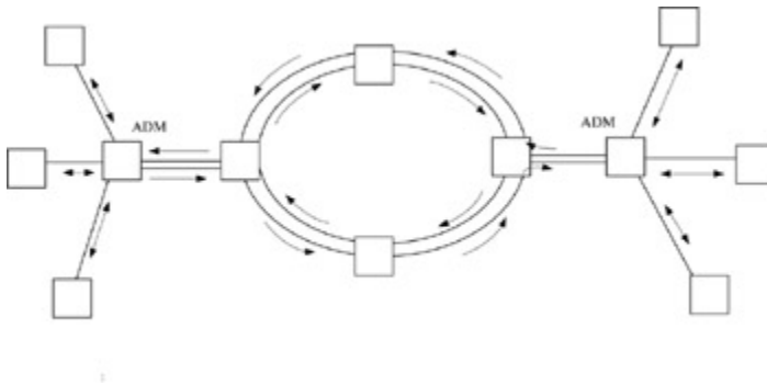
Figure 27-14: Ring architecture of SONET multiplexers
