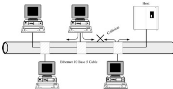
Figure 14-1: CSMA/CD cable networks are collision domains
