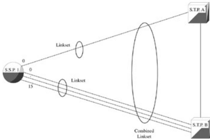
Figure 7-8: Linksets combined
