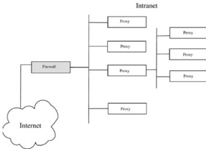
Figure 31-4: A typical array of proxy devices sitting behind the firewall
