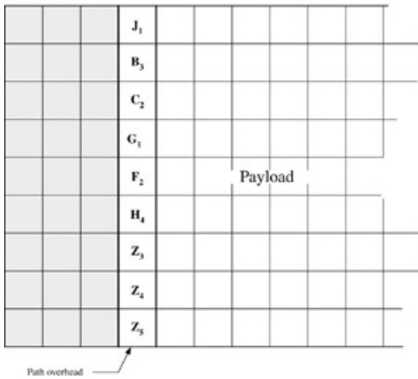
Figure 27-8: Path Overhead in the STS frame
