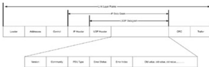
Figure 32-6: The SNMP message carried within the protocol layers
