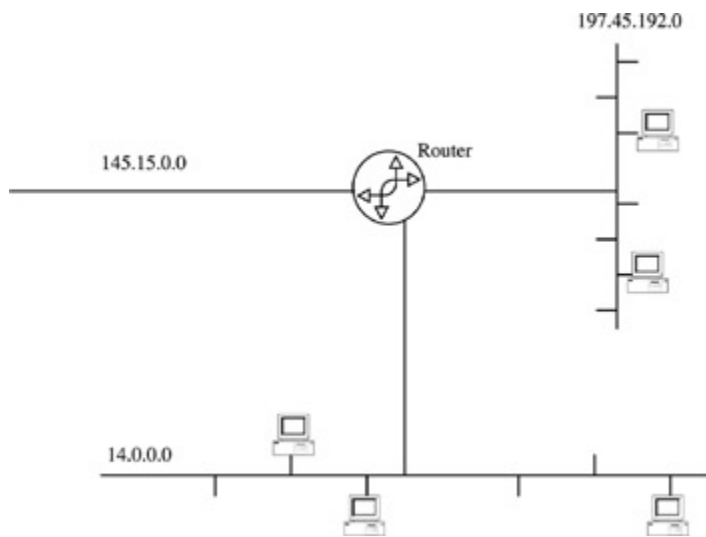
Figure 29-10: Different classes of IP addresses connected to a router
