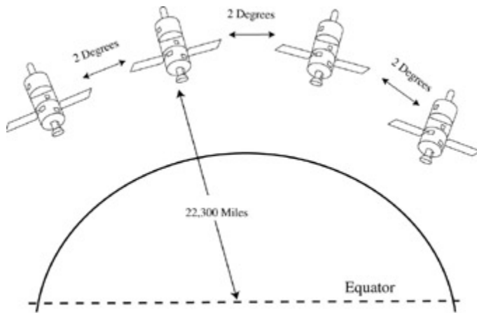
Figure 24-4: Geosynchronous Orbit
