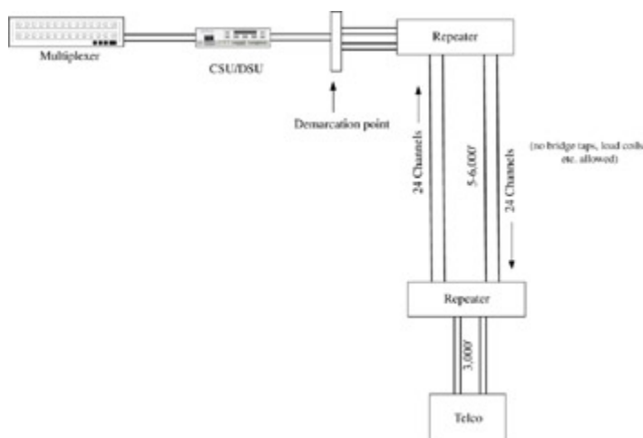
Figure 16-3: The typical layout of the T1
