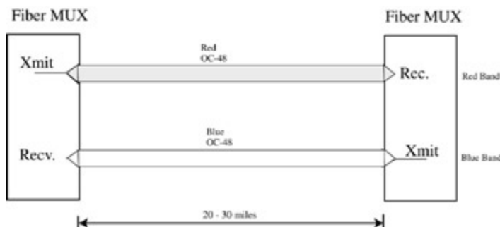
Figure 28-2: The colors of light separate the bands carried on the cable
