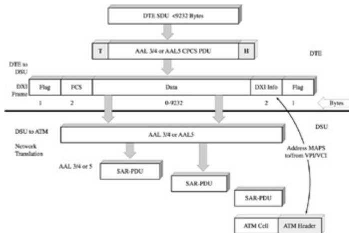
Figure 12-17: DXI protocol mode 1B
