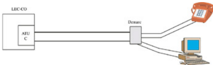
Figure 16-8: The splitterless G.Lite installation
