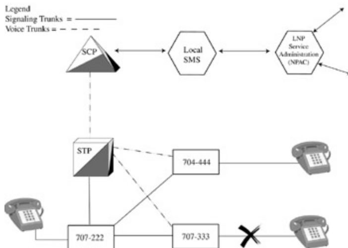
Figure 5-2: Basic LNP network
