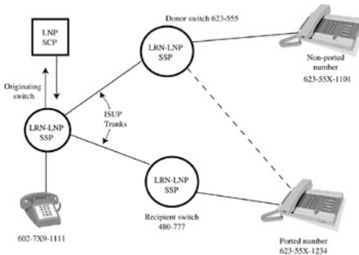
Figure 5-3: LNP terminology
