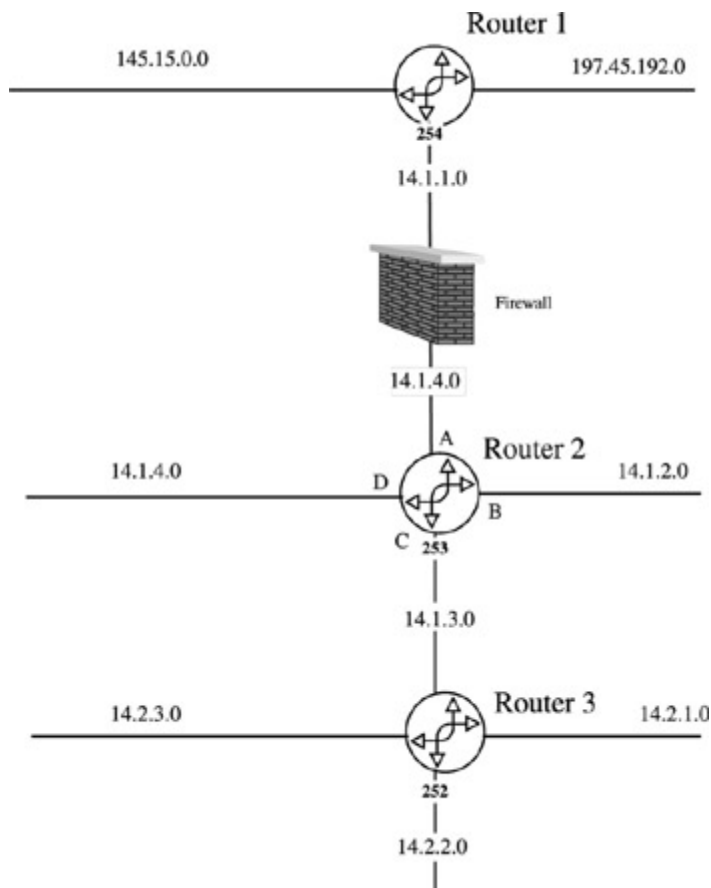
Figure 29-12: Class A subnetted with a firewall to the Internet
