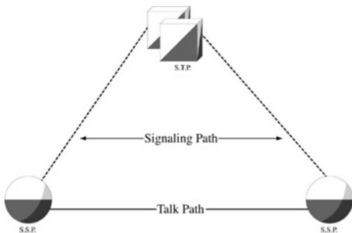
Figure 7-6: Quasi-associated signaling
