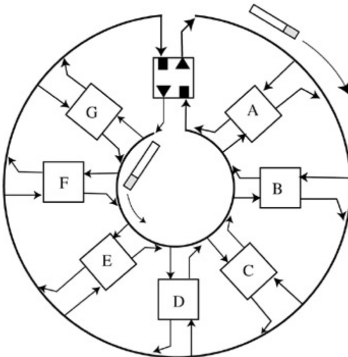
Figure 9-10: The distributed queue dual bus (DQDB) system.
