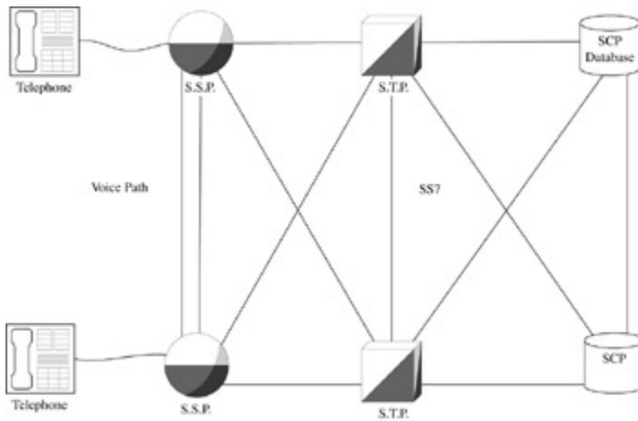
Figure 7-3: SS7 architectural beginnings
