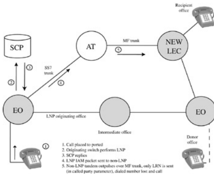
Figure 5-5: LNP scenario
