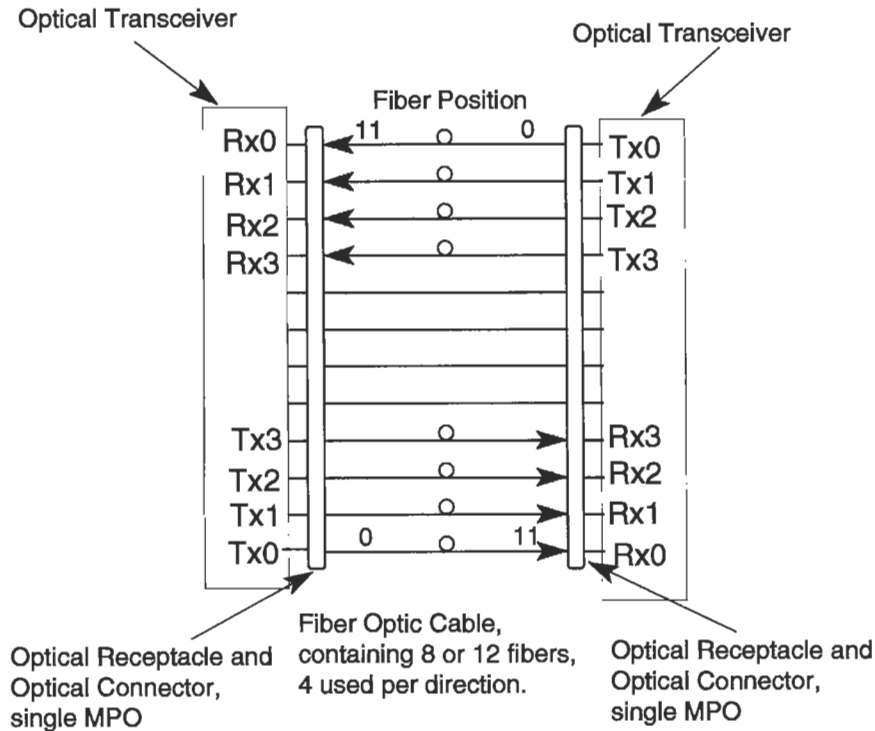
Fig. 9.9 4X-SX Fiber Optic Link Configuration.
