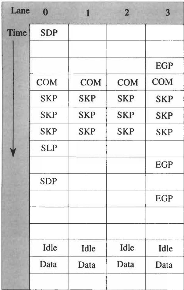
Fig. 9.2 Shows structure of data format as it gets striped across 4 lanes.
