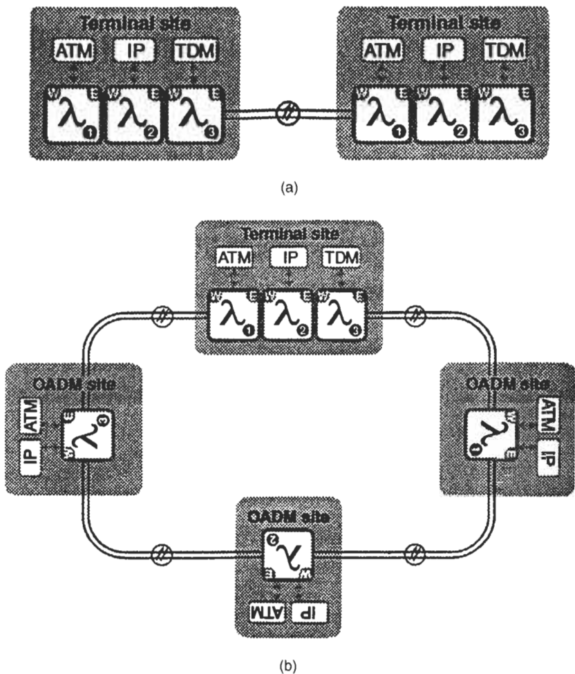
Fig. 5.6 WDM network topologies (a) point-to-point (b) hubbed ring.
