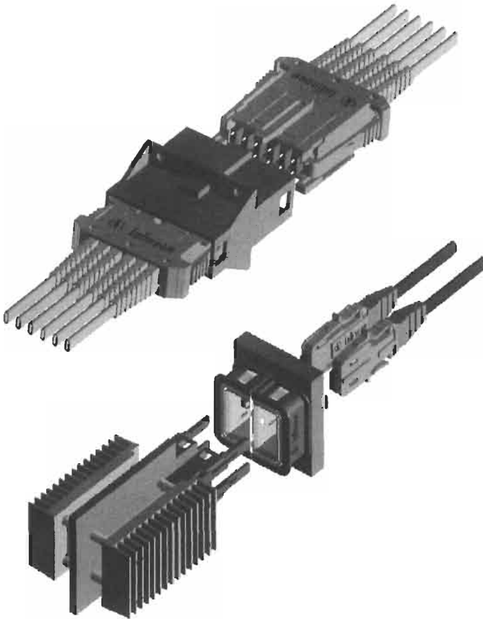
Fig. 6.11 Infineon's MMC TM (Multi MC) connector and adapter system for up to 6 MT connectors with 12 fibers each at 250- \mu m pitch (top) and PAROLI transmitter and receiver arrangement for direct coupling into a duplex-type backplane connection module [70a] (bottom).
