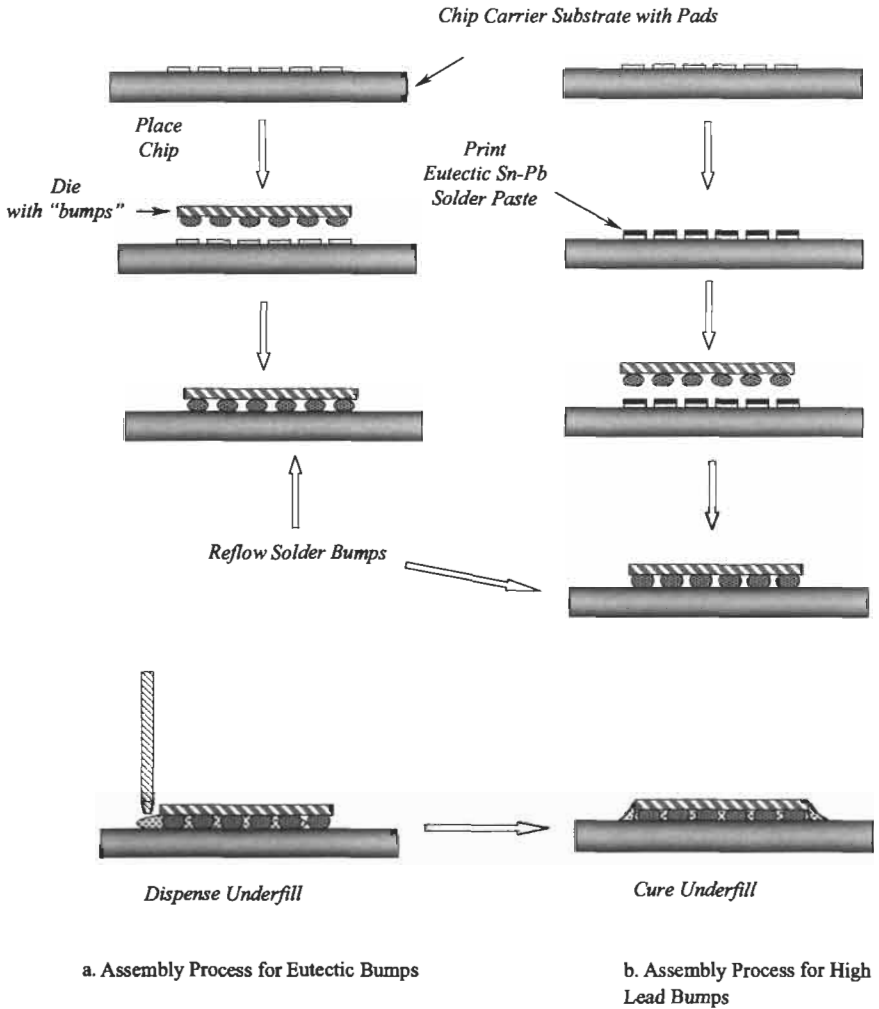
Fig. 8.6 Flip Chip Assembly Process.
