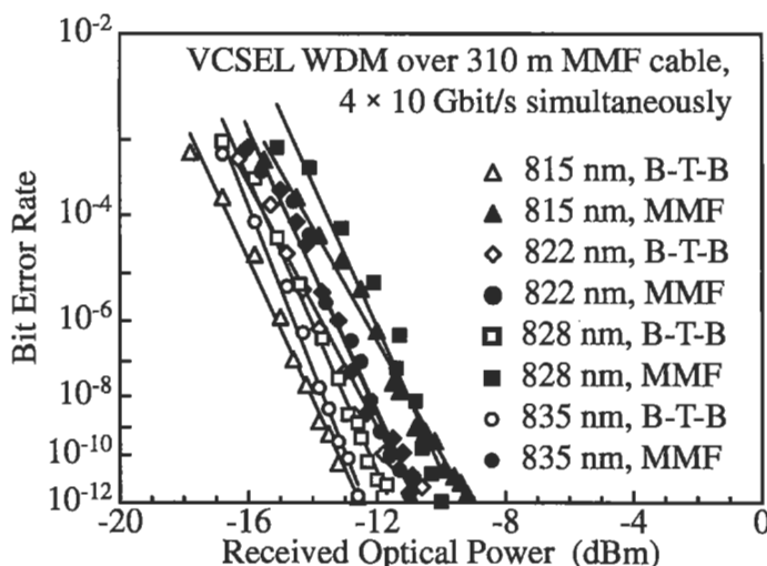
Fig. 6.7 Bit error rates in a 4-channel CWDM experiment showing 4 \times 10 Gbit/s data transmission over 310 m of a 50- \mu m core diameter MMF cable [41].
