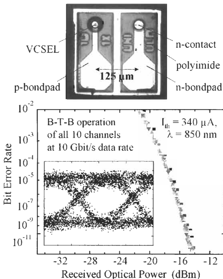
Fig. 6.2 Cleaved unit cell of a linear 1 × 10, 250-μm spacing VCSEL array with coplanar, 125-μm pitch contact arrangement (top) and bit error rate characteristics for back-to-back (B-T-B) operation of all 10 channels at 10 Gbit/s modulation with a representative eye diagram (on a 200 ps horizontal and 900 mV vertical scale) in the inset (bottom).
