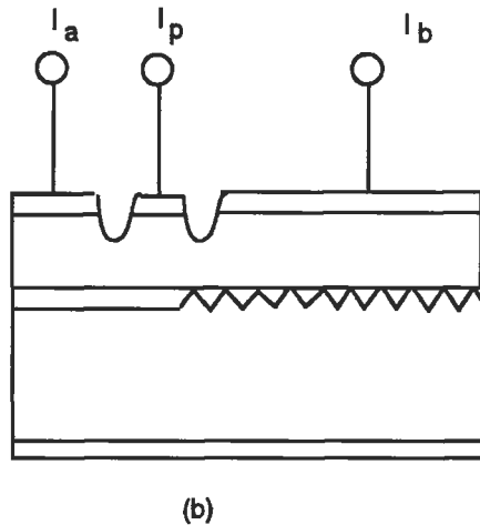
Fig. 11.4 Structure of a (a) two-section (b) three-section laser diode.
