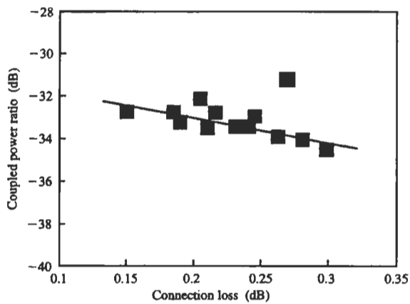
Fig. 4.10 Coupled optical power vs MCP connection loss.
