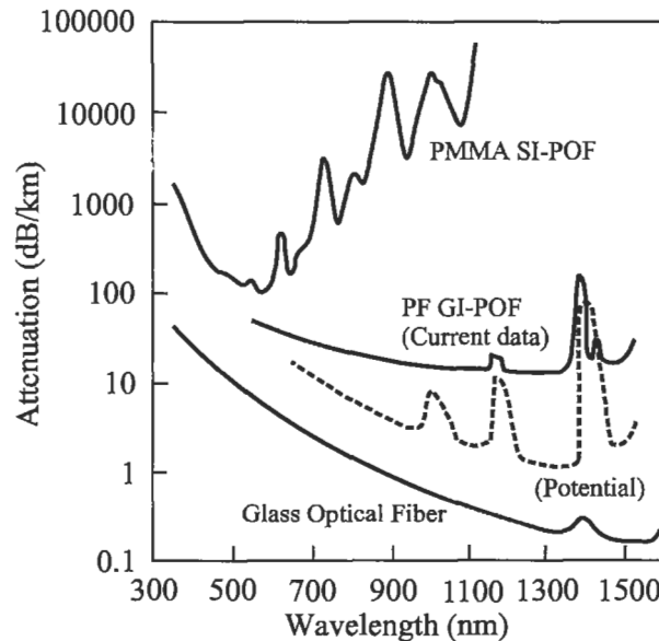
Fig. 6.8 Currently achieved as well as potential attenuation characteristics of a perfluorinated polymer (CYTOP) fiber compared with standard silica glass and polymethyl methacrylate (PMMA) material [46].
