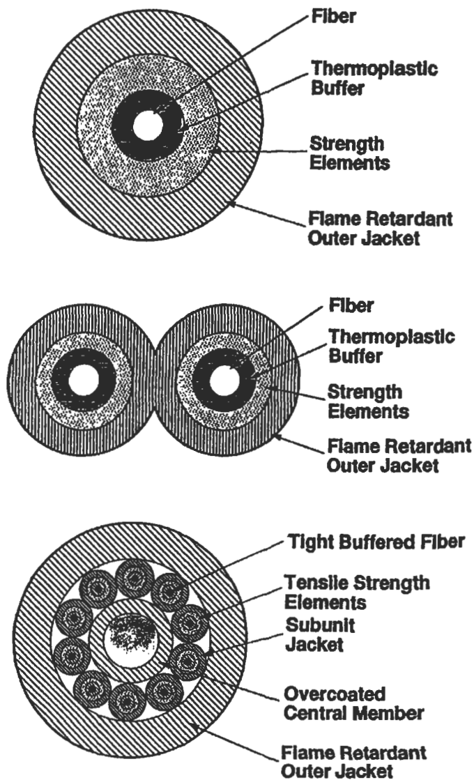
Fig. 4.2 Different types of fiber optic cable cross-sections.
